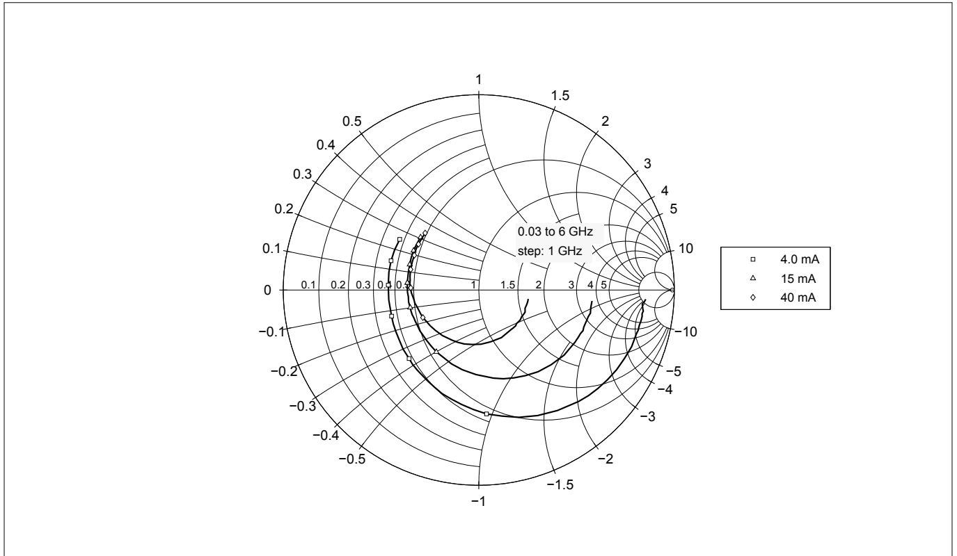
Figure 17 Input reflection coefficient S_{11} = f(f) , V_{CE} = 3V , I_C = 4 / 15 / 40\text{ mA}
