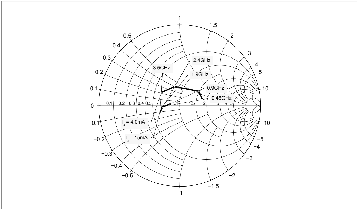
Figure 18 Source impedance for minimum noise figure Z_{S,opt} = f(f) , V_{CE} = 3V , I_C = 4 / 15\text{ mA}
